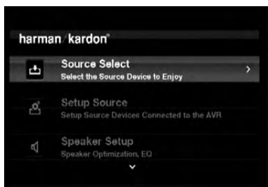
Figure 19 – Main Menu
