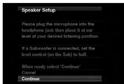
Figure 21 – EzSet/EQ Screen
