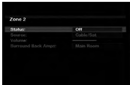
Figure 38 – Zone 2 Menu
